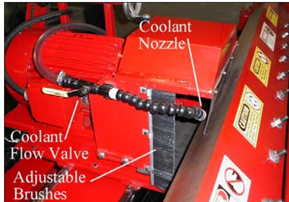
Horizontal Floor Model is a full flood coolant machine with adjustable nozzle and brushed to direct flow and control splatter.
